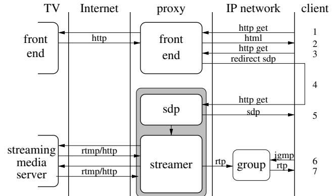
Fig. 1. Schematic representation of the unicast/multicast proxy gateway.
